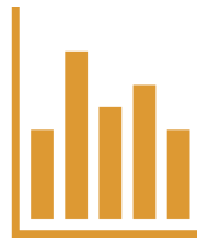
Data analysis
